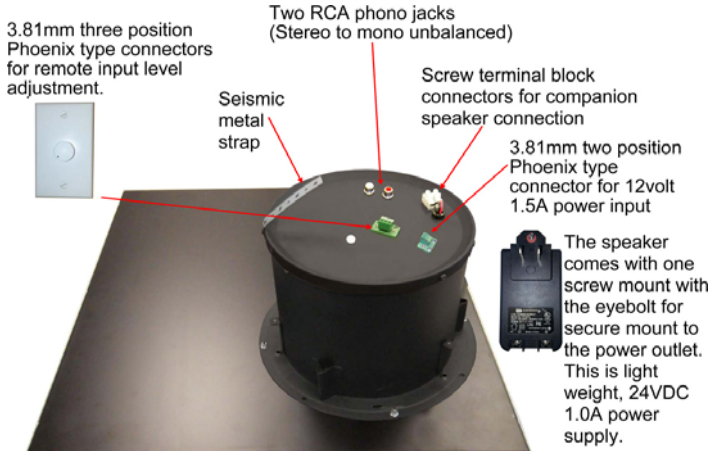
Powered Speaker
