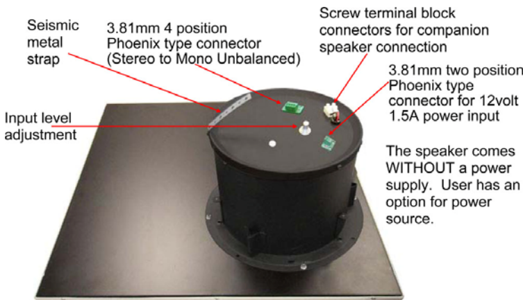
Powered Speaker
