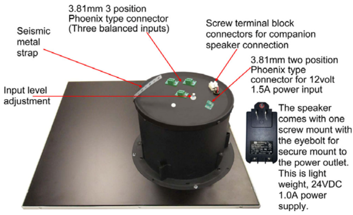
Powered Speaker
