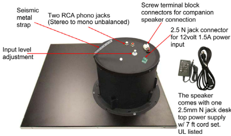
Powered Speaker
