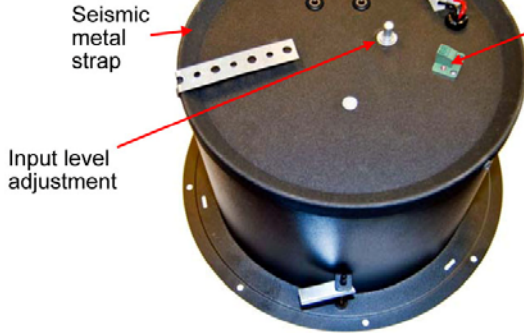
Powered Speaker
