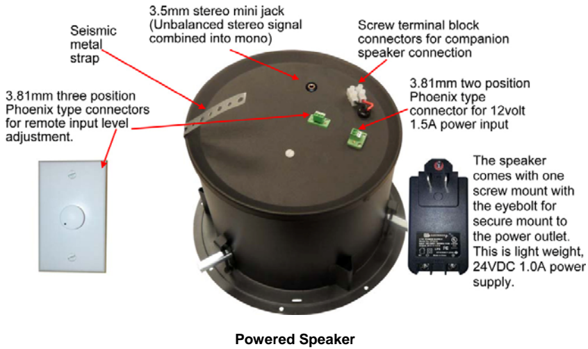
Powered Speaker
